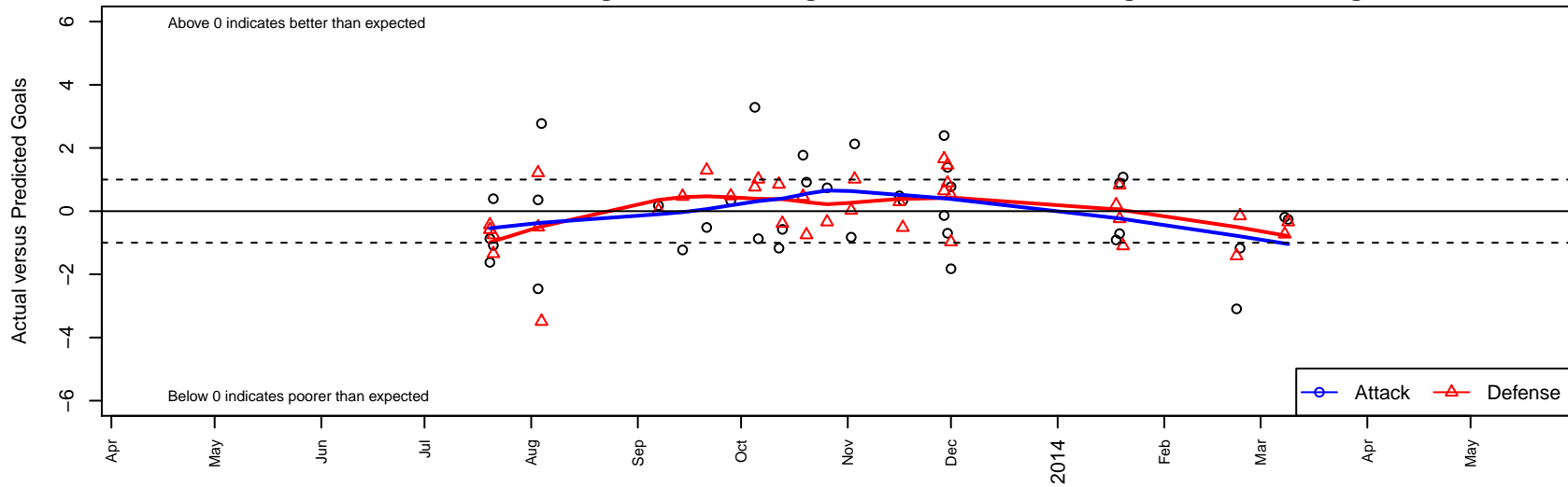
San Diego Surf SC Premier I B01 Dots are actual minus expected GF (blue circles) and GA (red triangles). Blue line is smoothed change in attack strength. Red is smoothed change in defense strength.
